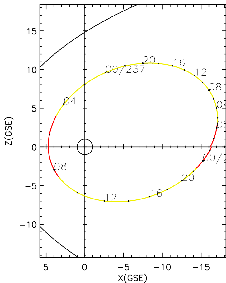
CLUSTER 2 orbit 2020 235 (08/22) 20:21 UT to 2020 238 (08/25) 02:36 UT
