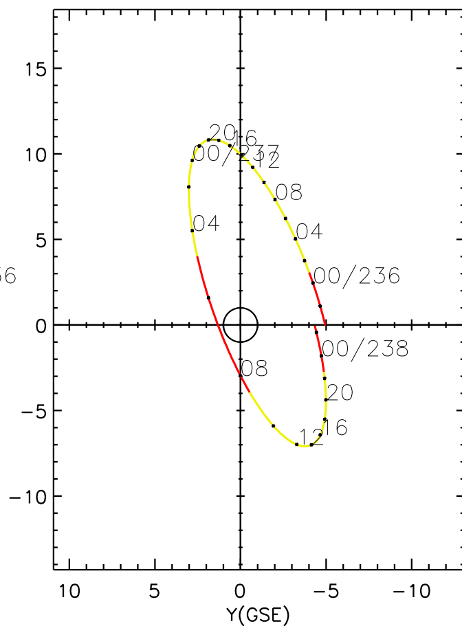
CLUSTER 2 orbit 2020 235 (08/22) 20:21 UT to 2020 238 (08/25) 02:36 UT
