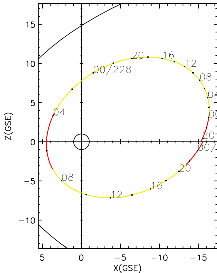
CLUSTER 2 orbit 2020 226 (08/13) 19:21 UT to 2020 229 (08/16) 01:36 UT
