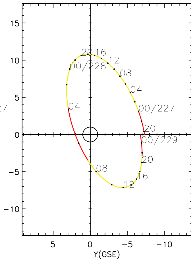
CLUSTER 2 orbit 2020 226 (08/13) 19:21 UT to 2020 229 (08/16) 01:36 UT
