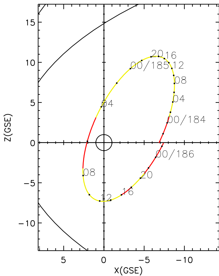
CLUSTER 2 orbit 2020 183 (07/01) 20:21 UT to 2020 186 (07/04) 02:36 UT
