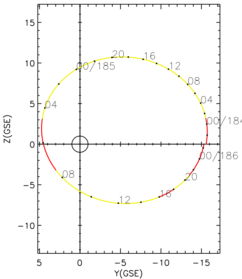
CLUSTER 2 orbit 2020 183 (07/01) 20:21 UT to 2020 186 (07/04) 02:36 UT
