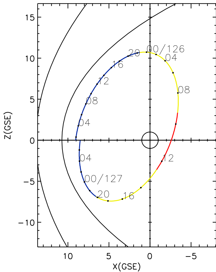
CLUSTER 2 orbit 2020 125 (05/04) 01:26 UT to 2020 127 (05/06) 07:41 UT
