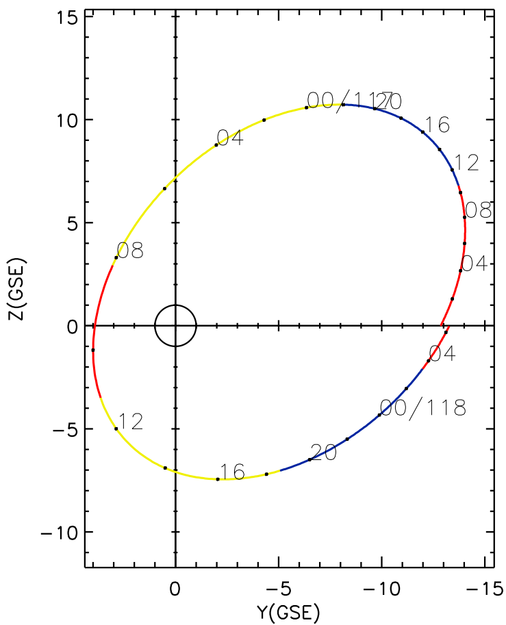
CLUSTER 2 orbit 2020 116 (04/25) 00:06 UT to 2020 118 (04/27) 06:26 UT
