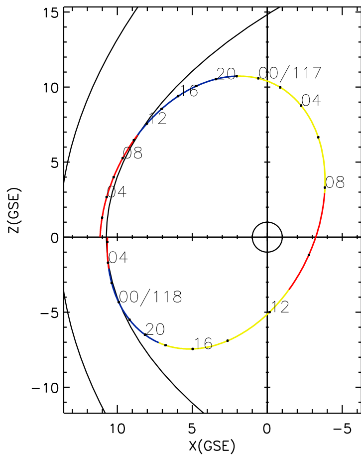
CLUSTER 2 orbit 2020 116 (04/25) 00:06 UT to 2020 118 (04/27) 06:26 UT
