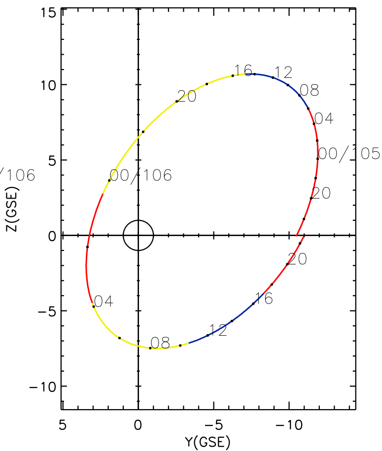
CLUSTER 2 orbit 2020 104 (04/13) 16:21 UT to 2020 106 (04/15) 22:41 UT
