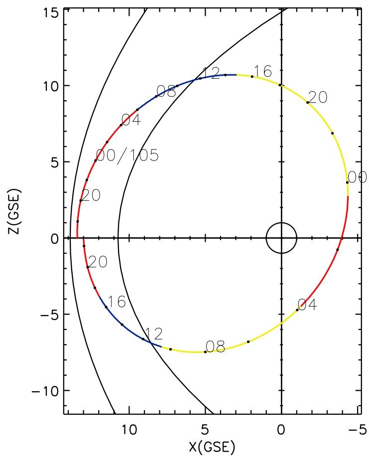
CLUSTER 2 orbit 2020 104 (04/13) 16:21 UT to 2020 106 (04/15) 22:41 UT
