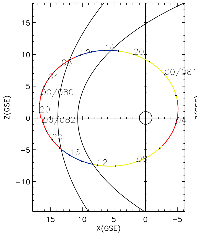
CLUSTER 2 orbit 2020 079 (03/19) 18:41 UT to 2020 082 (03/22) 01:01 UT
