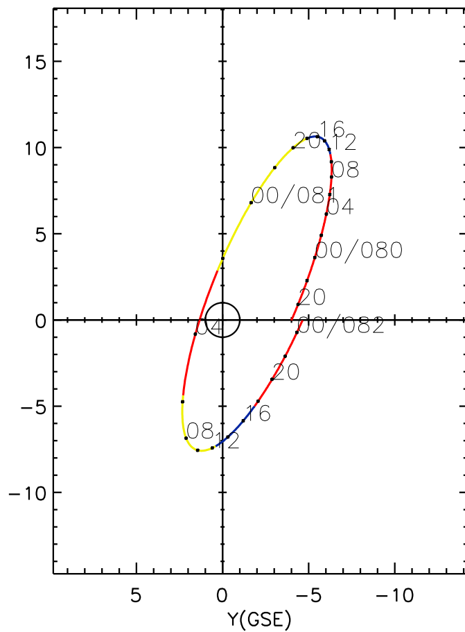
CLUSTER 2 orbit 2020 079 (03/19) 18:41 UT to 2020 082 (03/22) 01:01 UT
