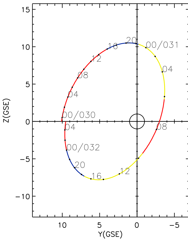
CLUSTER 2 orbit 2020 029 (01/29) 23:16 UT to 2020 032 (02/01) 05:36 UT
