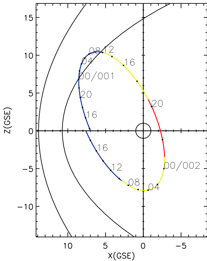
CLUSTER 2 orbit 2019 365 (12/31) 13:31 UT to 2020 002 (01/02) 19:46 UT
