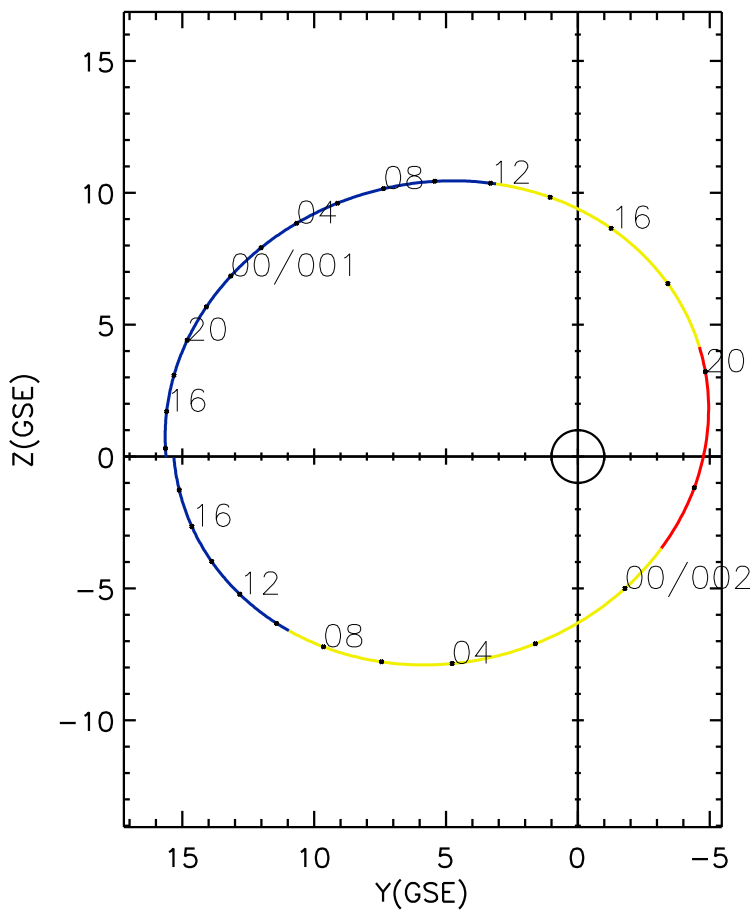
CLUSTER 2 orbit 2019 365 (12/31) 13:31 UT to 2020 002 (01/02) 19:46 UT
