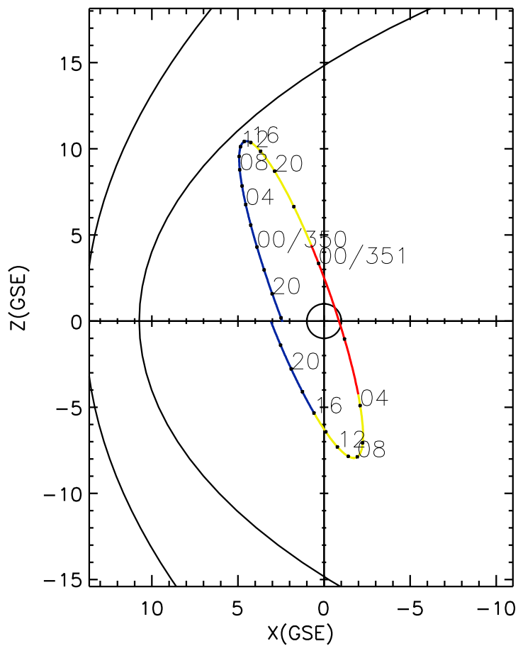
CLUSTER 2 orbit 2019 349 (12/15) 17:41 UT to 2019 351 (12/17) 23:56 UT
