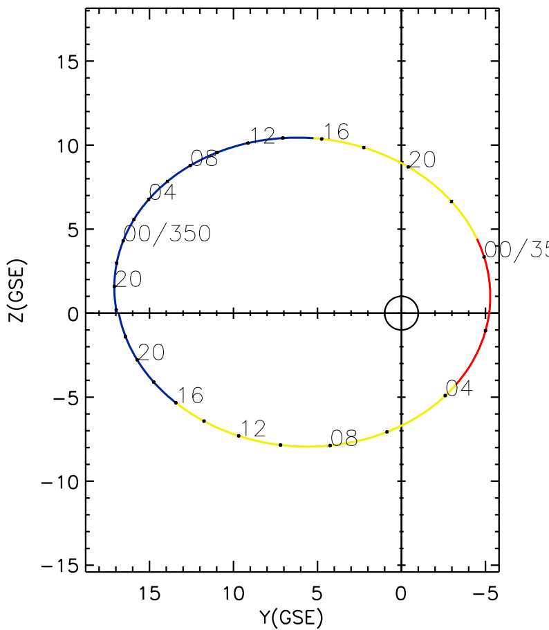
CLUSTER 2 orbit 2019 349 (12/15) 17:41 UT to 2019 351 (12/17) 23:56 UT
