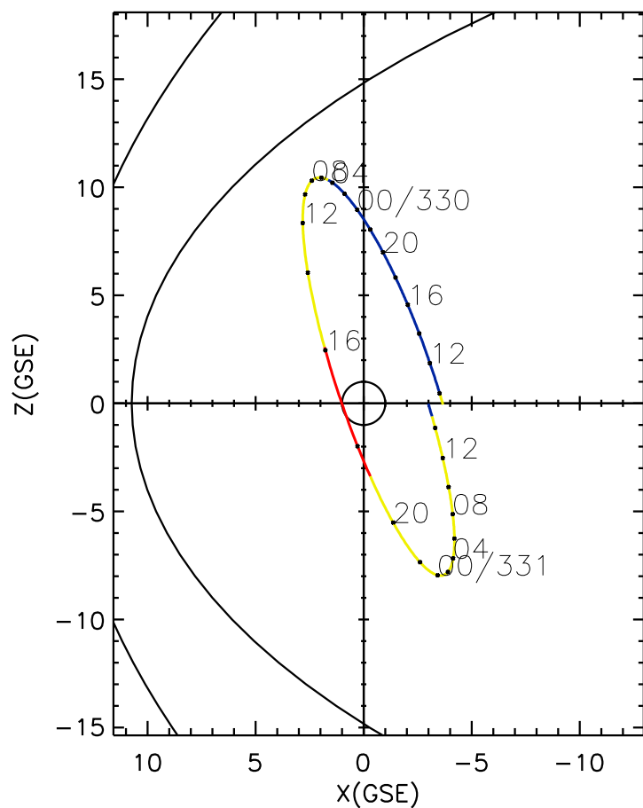
CLUSTER 2 orbit 2019 329 (11/25) 09:16 UT to 2019 331 (11/27) 15:36 UT
