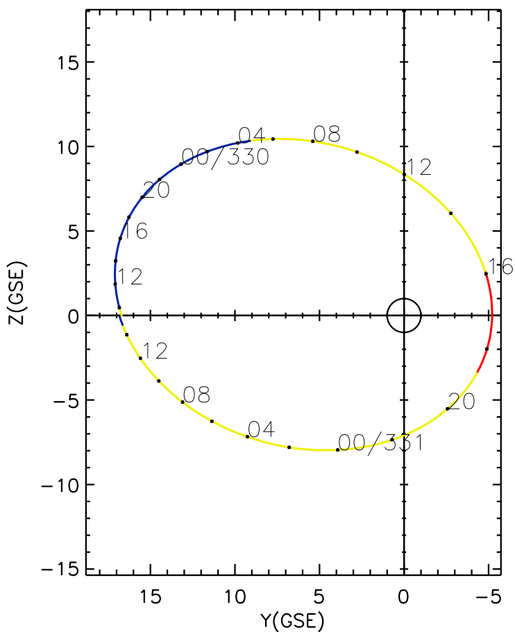
CLUSTER 2 orbit 2019 329 (11/25) 09:16 UT to 2019 331 (11/27) 15:36 UT
