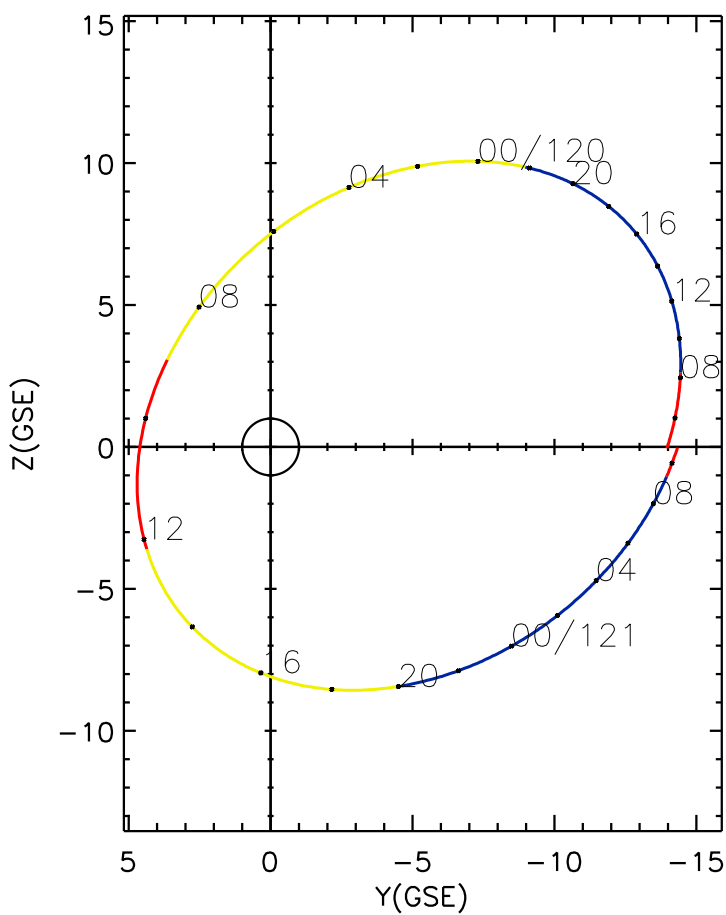
CLUSTER 2 orbit 2019 119 (04/29) 04:31 UT to 2019 121 (05/01) 10:46 UT
