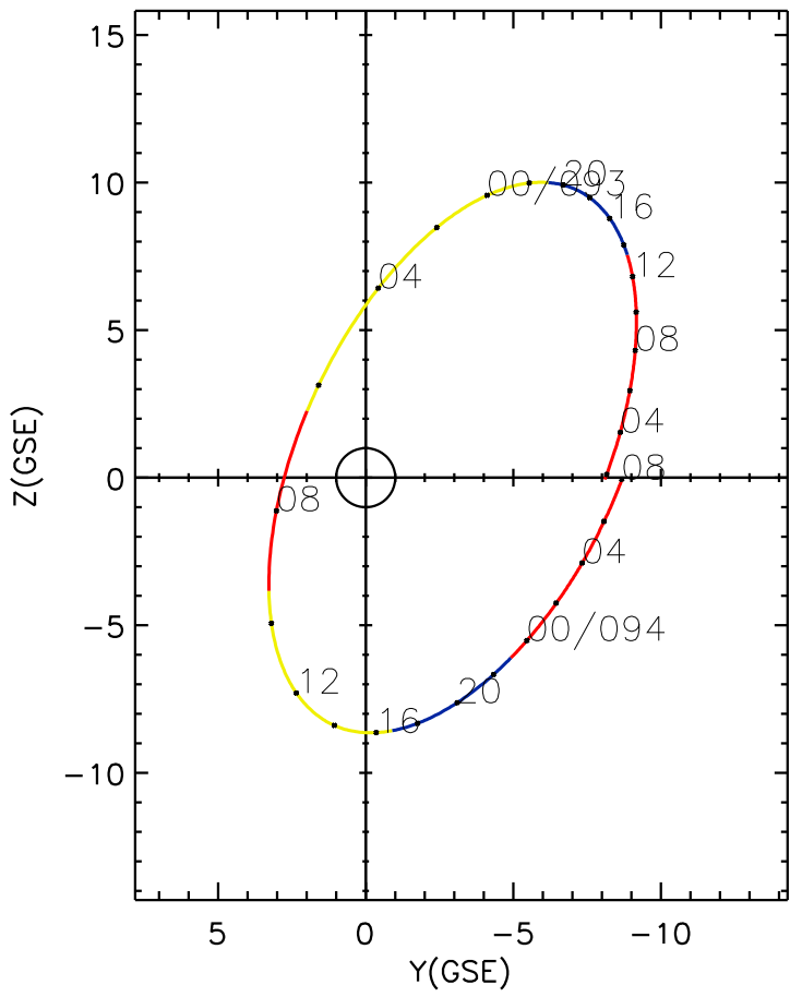
CLUSTER 2 orbit 2019 092 (04/02) 01:46 UT to 2019 094 (04/04) 08:01 UT
