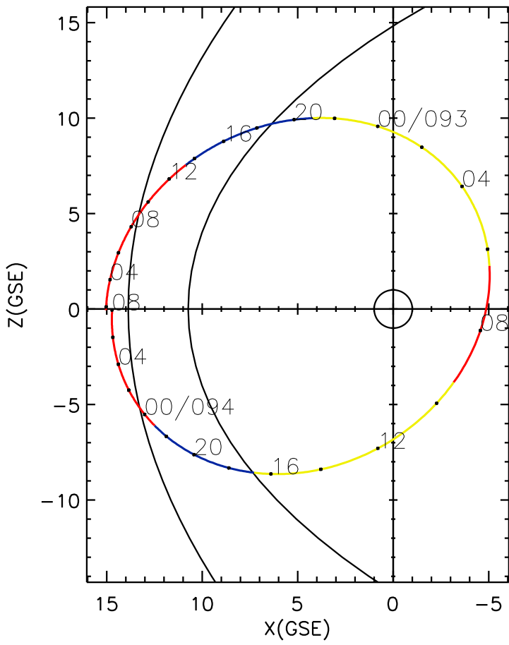
CLUSTER 2 orbit 2019 092 (04/02) 01:46 UT to 2019 094 (04/04) 08:01 UT
