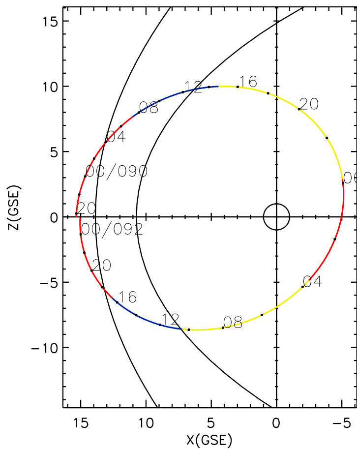
CLUSTER 2 orbit 2019 089 (03/30) 19:36 UT to 2019 092 (04/02) 01:46 UT
