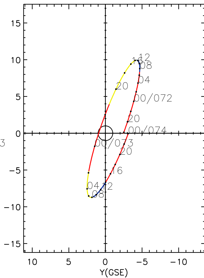
CLUSTER 2 orbit 2019 071 (03/12) 17:46 UT to 2019 074 (03/15) 00:01 UT
