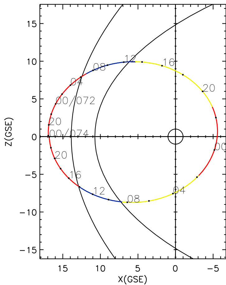
CLUSTER 2 orbit 2019 071 (03/12) 17:46 UT to 2019 074 (03/15) 00:01 UT
