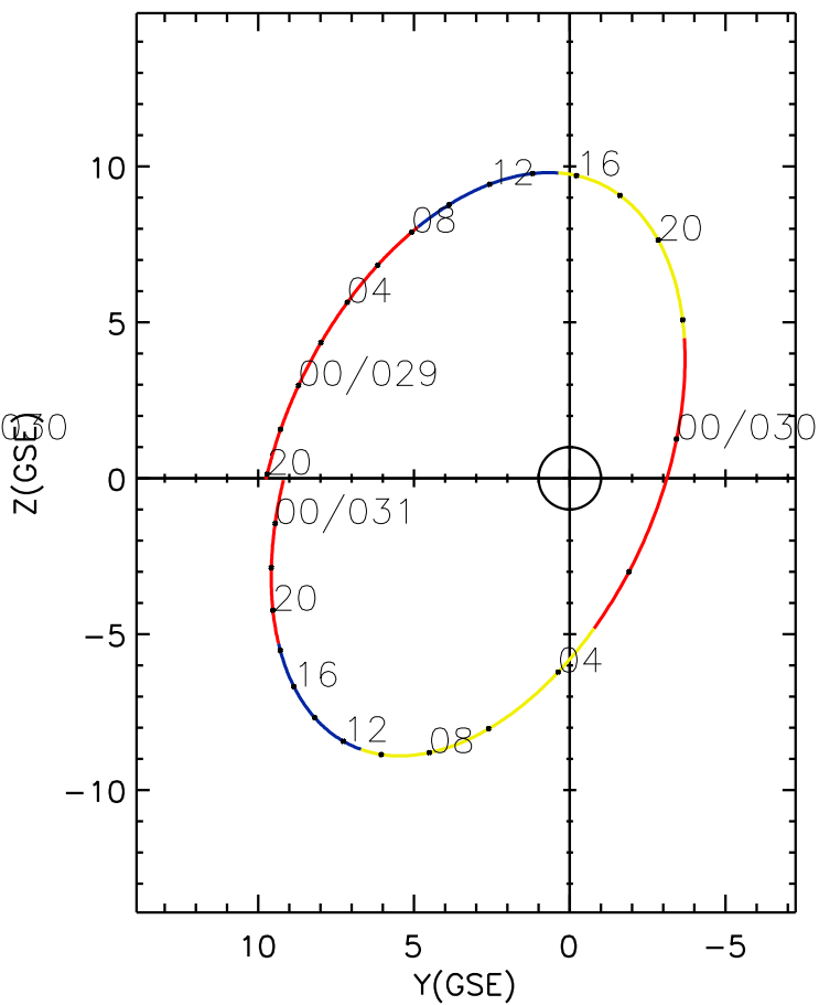
CLUSTER 2 orbit 2019 028 (01/28) 19:46 UT to 2019 031 (01/31) 01:56 UT
