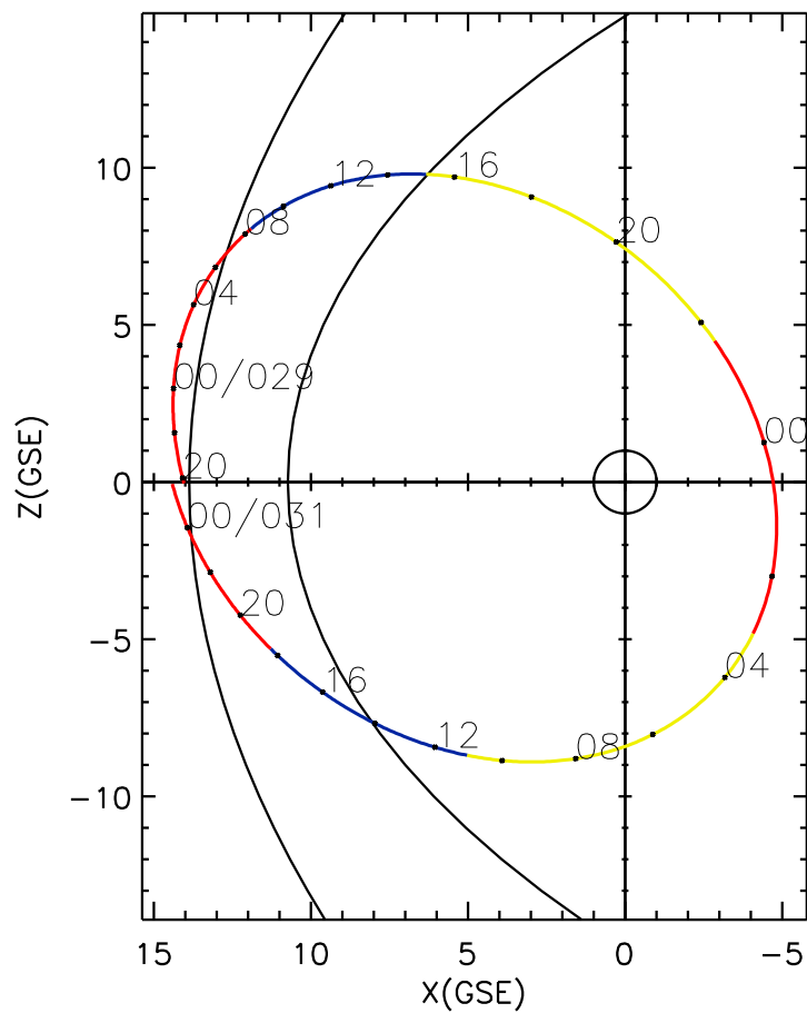
CLUSTER 2 orbit 2019 028 (01/28) 19:46 UT to 2019 031 (01/31) 01:56 UT
