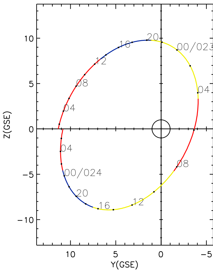
CLUSTER 2 orbit 2019 022 (01/22) 01:16 UT to 2019 024 (01/24) 07:26 UT
