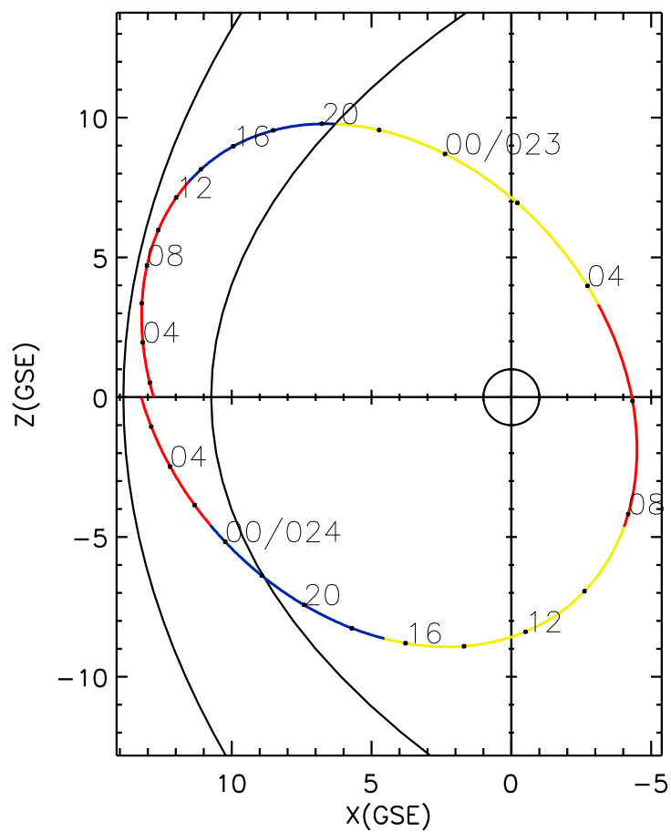
CLUSTER 2 orbit 2019 022 (01/22) 01:16 UT to 2019 024 (01/24) 07:26 UT
