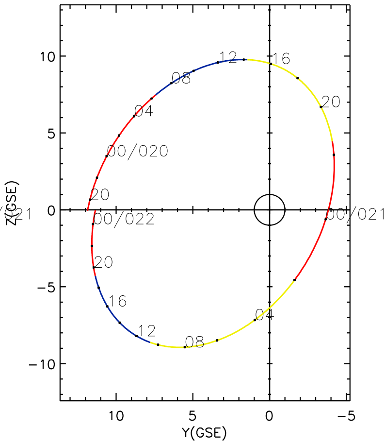
CLUSTER 2 orbit 2019 019 (01/19) 19:01 UT to 2019 022 (01/22) 01:16 UT
