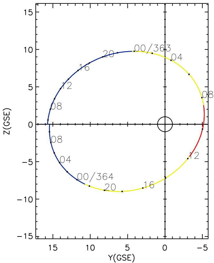
CLUSTER 2 orbit 2018 362 (12/28) 05:11 UT to 2018 364 (12/30) 11:21 UT
