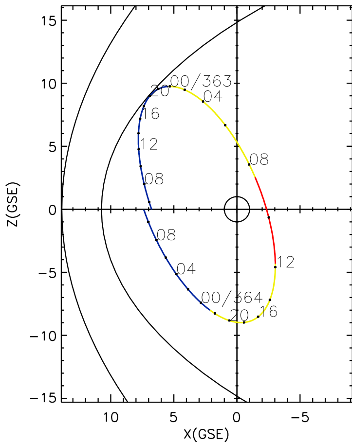
CLUSTER 2 orbit 2018 362 (12/28) 05:11 UT to 2018 364 (12/30) 11:21 UT
