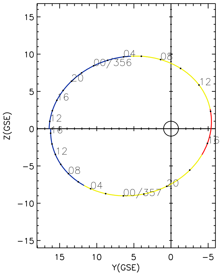
CLUSTER 2 orbit 2018 355 (12/21) 10:36 UT to 2018 357 (12/23) 16:46 UT
