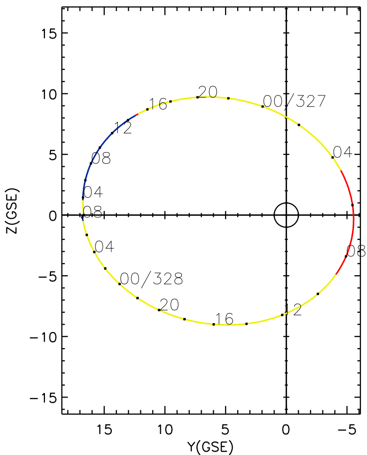
CLUSTER 2 orbit 2018 326 (11/22) 01:56 UT to 2018 328 (11/24) 08:11 UT
