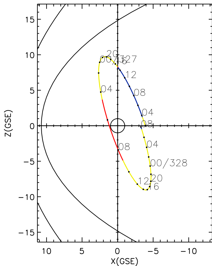
CLUSTER 2 orbit 2018 326 (11/22) 01:56 UT to 2018 328 (11/24) 08:11 UT
