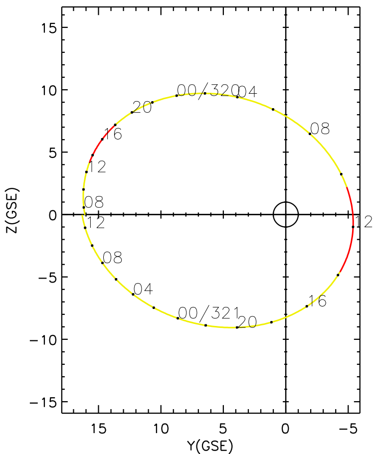
CLUSTER 2 orbit 2018 319 (11/15) 07:11 UT to 2018 321 (11/17) 13:26 UT
