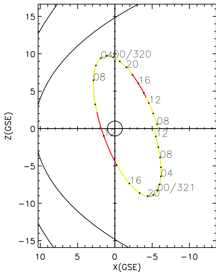
CLUSTER 2 orbit 2018 319 (11/15) 07:11 UT to 2018 321 (11/17) 13:26 UT
