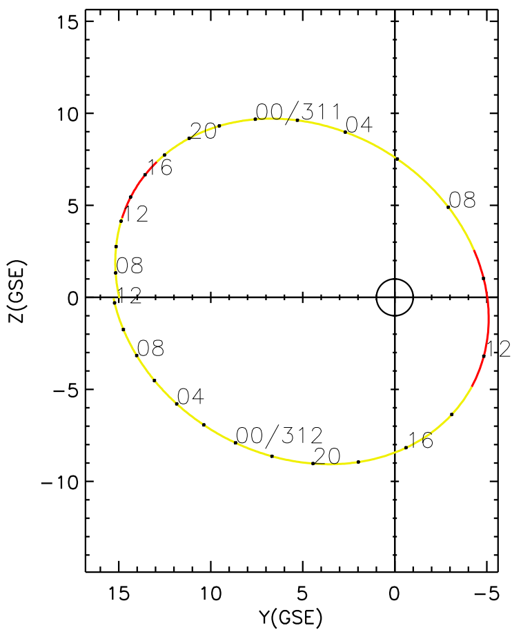
CLUSTER 2 orbit 2018 310 (11/06) 06:06 UT to 2018 312 (11/08) 12:21 UT
