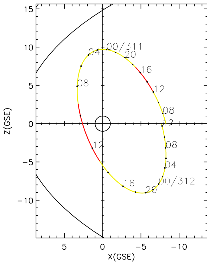
CLUSTER 2 orbit 2018 310 (11/06) 06:06 UT to 2018 312 (11/08) 12:21 UT
