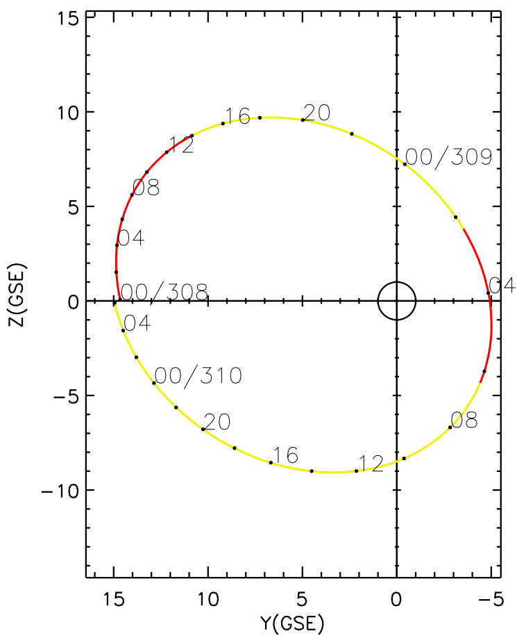
CLUSTER 2 orbit 2018 307 (11/03) 23:51 UT to 2018 310 (11/06) 06:06 UT
