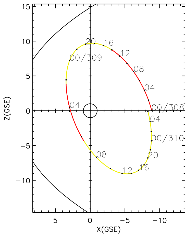
CLUSTER 2 orbit 2018 307 (11/03) 23:51 UT to 2018 310 (11/06) 06:06 UT
