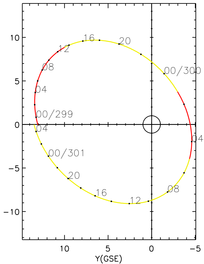
CLUSTER 2 orbit 2018 298 (10/25) 22:46 UT to 2018 301 (10/28) 05:06 UT
