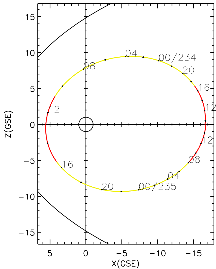
CLUSTER 2 orbit 2018 233 (08/21) 09:16 UT to 2018 235 (08/23) 15:36 UT
