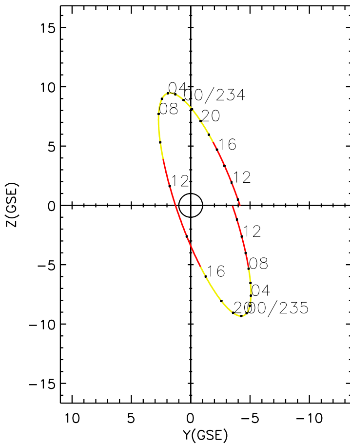
CLUSTER 2 orbit 2018 233 (08/21) 09:16 UT to 2018 235 (08/23) 15:36 UT
