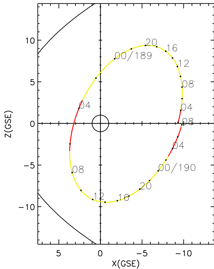
CLUSTER 2 orbit 2018 188 (07/07) 01:46 UT to 2018 190 (07/09) 08:11 UT
