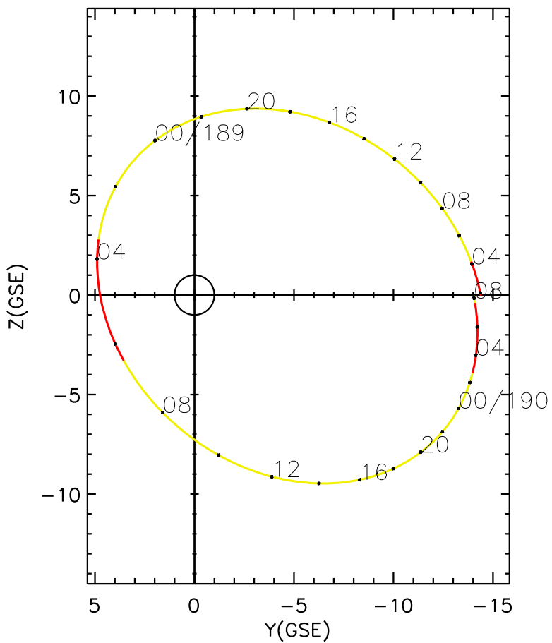
CLUSTER 2 orbit 2018 188 (07/07) 01:46 UT to 2018 190 (07/09) 08:11 UT
