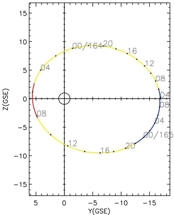
CLUSTER 2 orbit 2018 163 (06/12) 03:41 UT to 2018 165 (06/14) 10:01 UT
