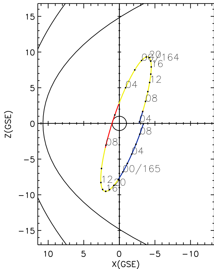
CLUSTER 2 orbit 2018 163 (06/12) 03:41 UT to 2018 165 (06/14) 10:01 UT
