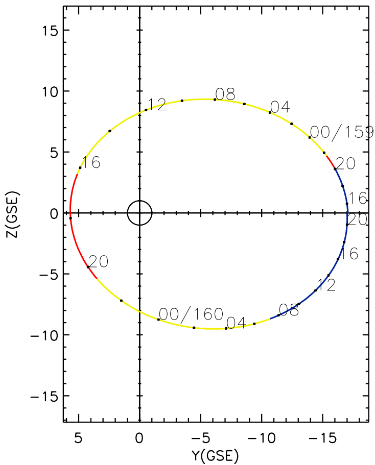
CLUSTER 2 orbit 2018 158 (06/07) 14:56 UT to 2018 160 (06/09) 21:16 UT
