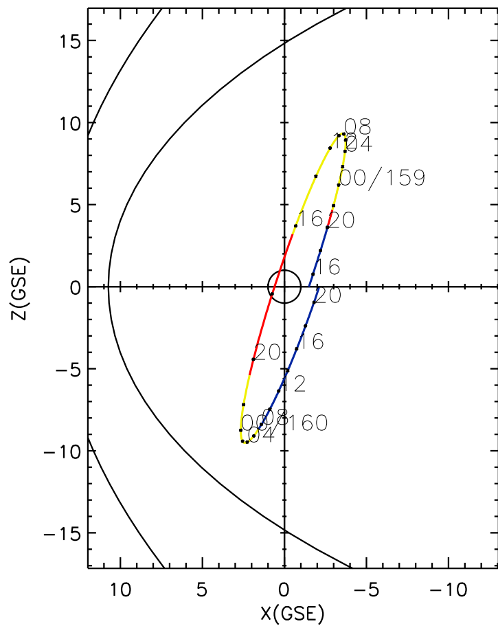
CLUSTER 2 orbit 2018 158 (06/07) 14:56 UT to 2018 160 (06/09) 21:16 UT
