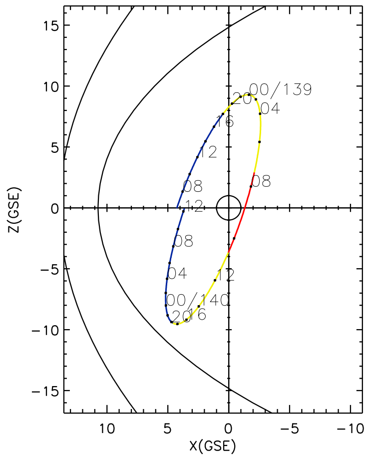
CLUSTER 2 orbit 2018 138 (05/18) 06:06 UT to 2018 140 (05/20) 12:21 UT
