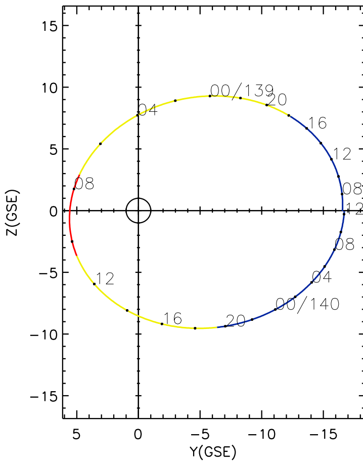
CLUSTER 2 orbit 2018 138 (05/18) 06:06 UT to 2018 140 (05/20) 12:21 UT
