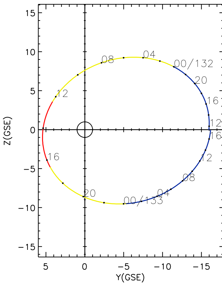
CLUSTER 2 orbit 2018 131 (05/11) 11:21 UT to 2018 133 (05/13) 17:36 UT
