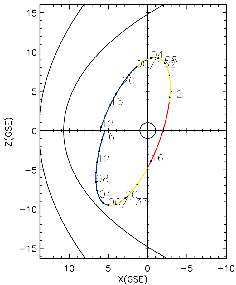
CLUSTER 2 orbit 2018 131 (05/11) 11:21 UT to 2018 133 (05/13) 17:36 UT
