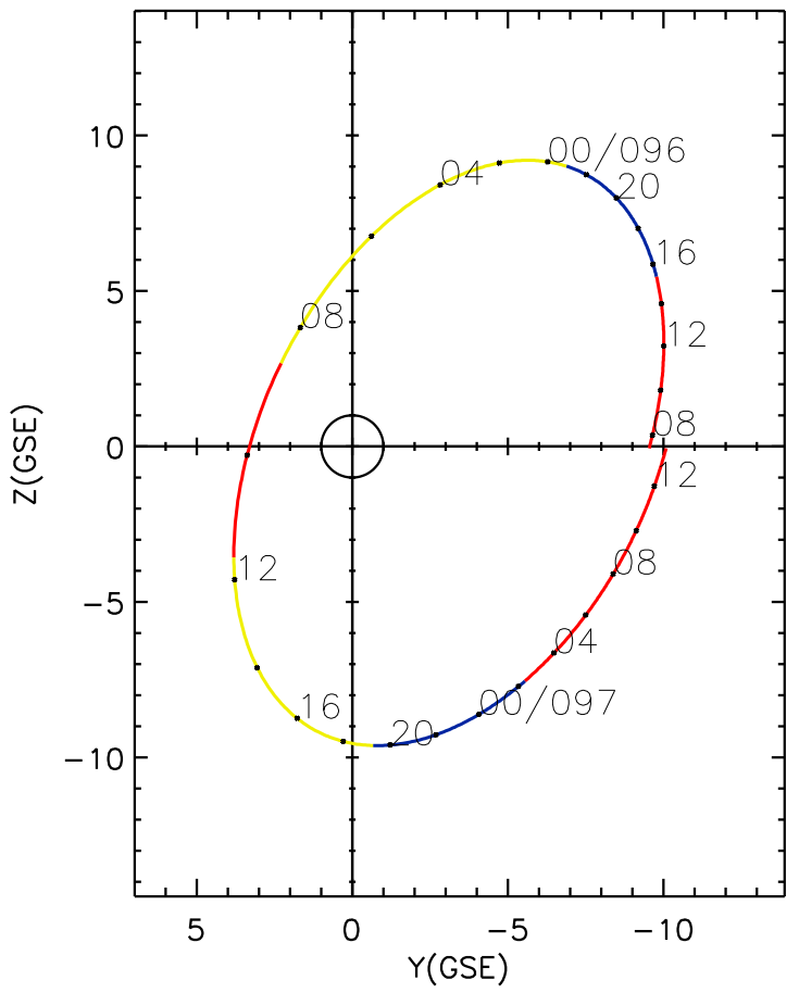
CLUSTER 2 orbit 2018 095 (04/05) 07:26 UT to 2018 097 (04/07) 13:41 UT
