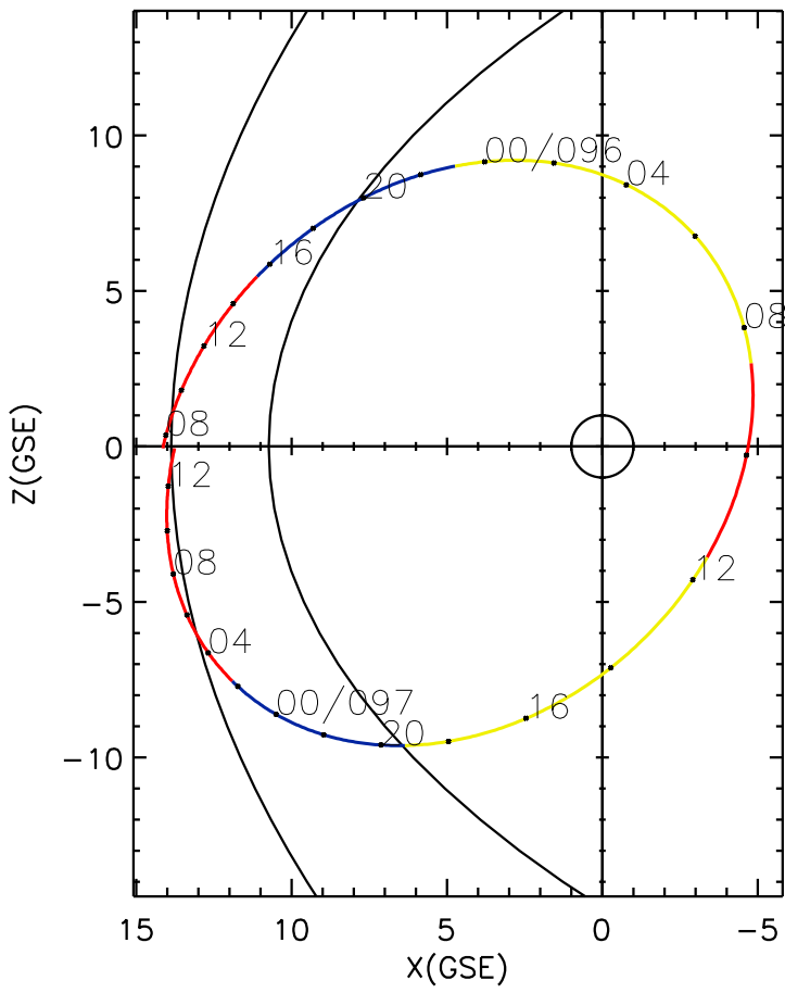
CLUSTER 2 orbit 2018 095 (04/05) 07:26 UT to 2018 097 (04/07) 13:41 UT
