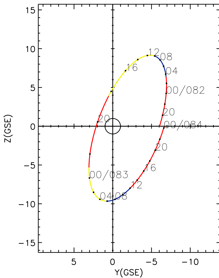
CLUSTER 2 orbit 2018 081 (03/22) 18:01 UT to 2018 084 (03/25) 00:16 UT
