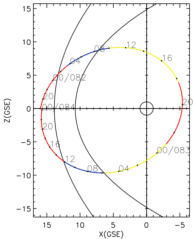
CLUSTER 2 orbit 2018 081 (03/22) 18:01 UT to 2018 084 (03/25) 00:16 UT
