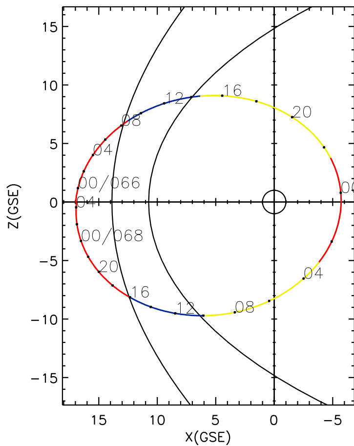
CLUSTER 2 orbit 2018 065 (03/06) 22:21 UT to 2018 068 (03/09) 04:36 UT
