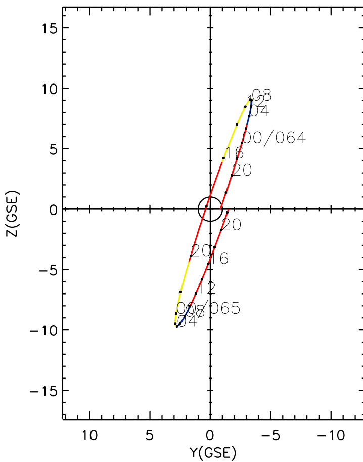
CLUSTER 2 orbit 2018 063 (03/04) 16:06 UT to 2018 065 (03/06) 22:21 UT
