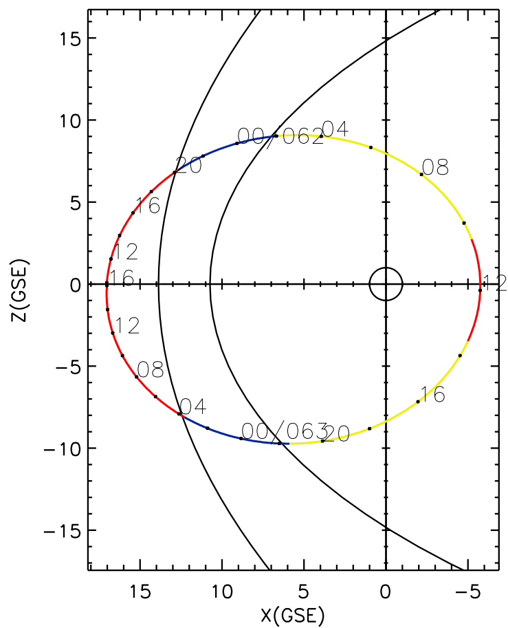
CLUSTER 2 orbit 2018 061 (03/02) 09:51 UT to 2018 063 (03/04) 16:06 UT
