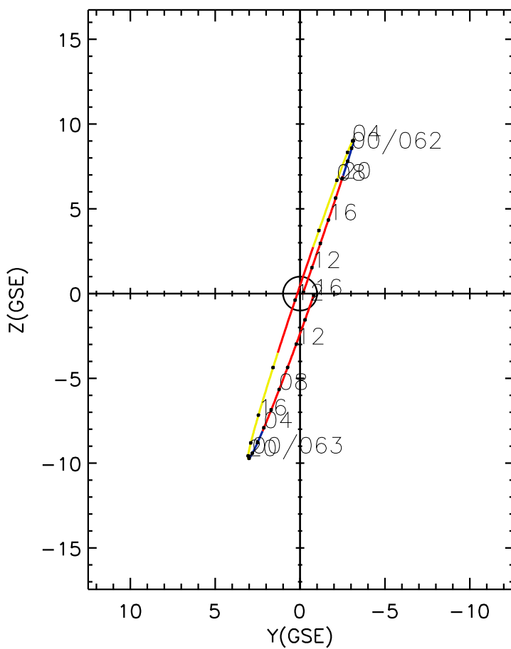
CLUSTER 2 orbit 2018 061 (03/02) 09:51 UT to 2018 063 (03/04) 16:06 UT
