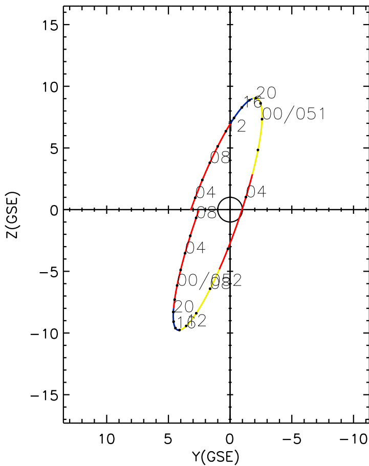
CLUSTER 2 orbit 2018 050 (02/19) 02:36 UT to 2018 052 (02/21) 08:51 UT
