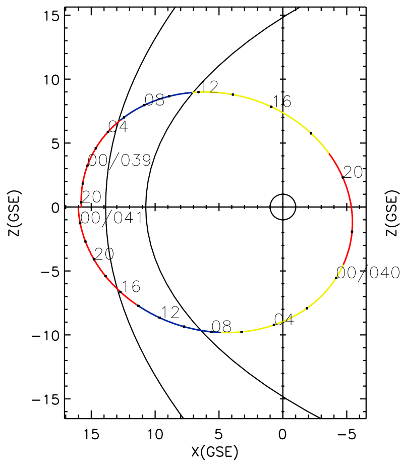
CLUSTER 2 orbit 2018 038 (02/07) 19:26 UT to 2018 041 (02/10) 01:41 UT
