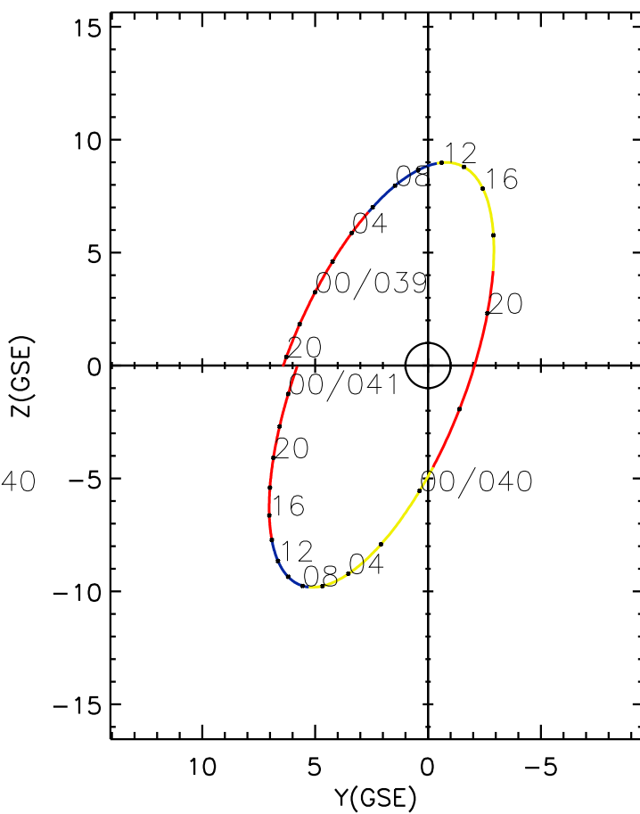
CLUSTER 2 orbit 2018 038 (02/07) 19:26 UT to 2018 041 (02/10) 01:41 UT
