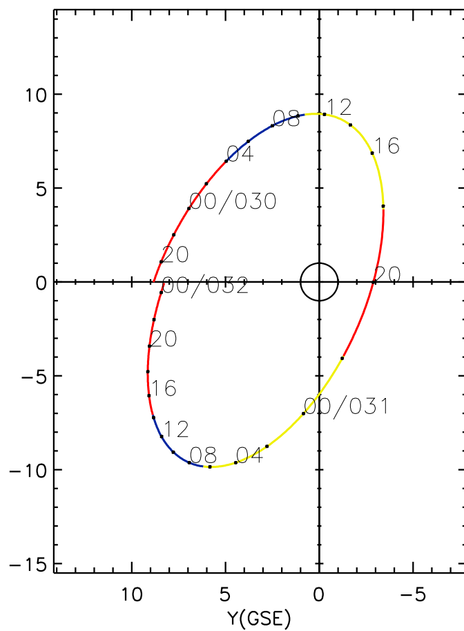
CLUSTER 2 orbit 2018 029 (01/29) 18:31 UT to 2018 032 (02/01) 00:41 UT
