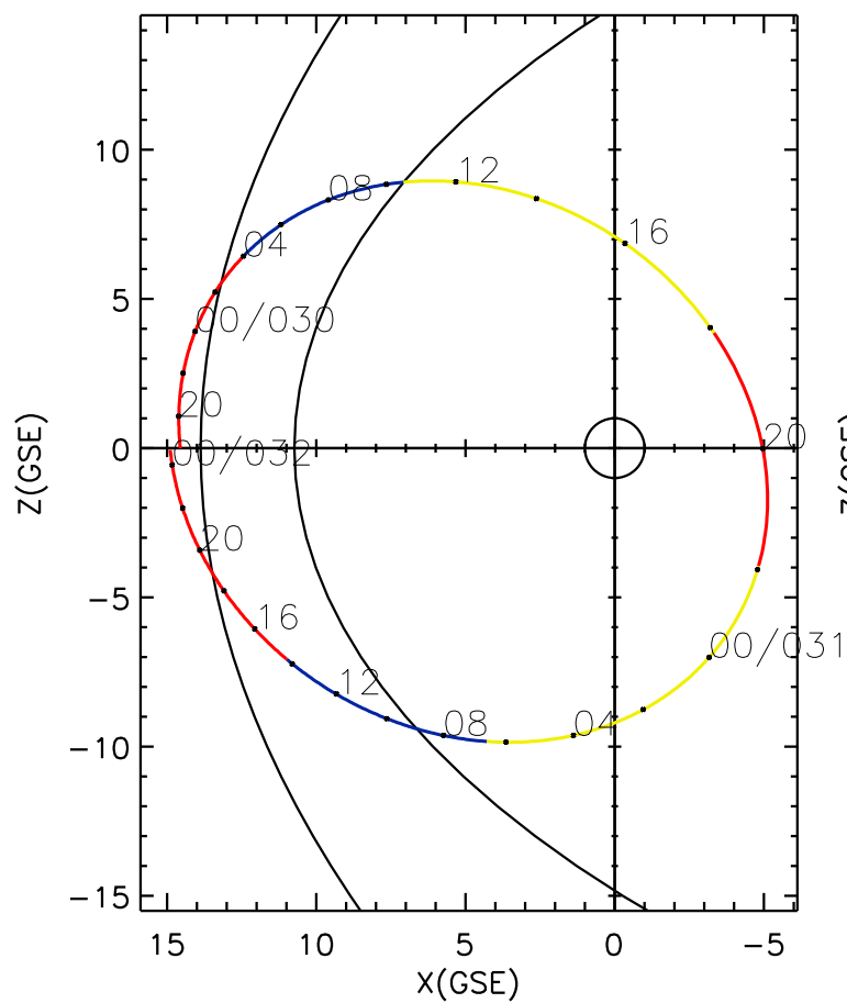
CLUSTER 2 orbit 2018 029 (01/29) 18:31 UT to 2018 032 (02/01) 00:41 UT
