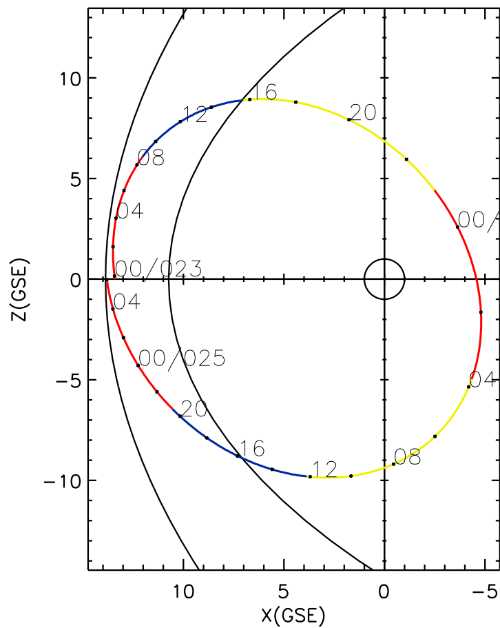
CLUSTER 2 orbit 2018 022 (01/22) 23:46 UT to 2018 025 (01/25) 06:01 UT
