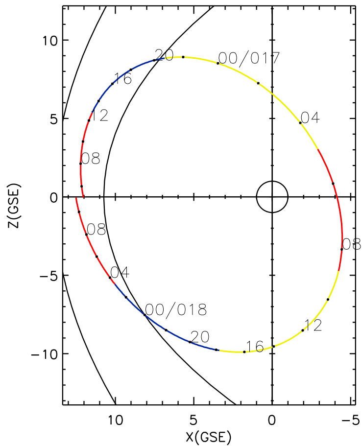
CLUSTER 2 orbit 2018 016 (01/16) 05:01 UT to 2018 018 (01/18) 11:16 UT
