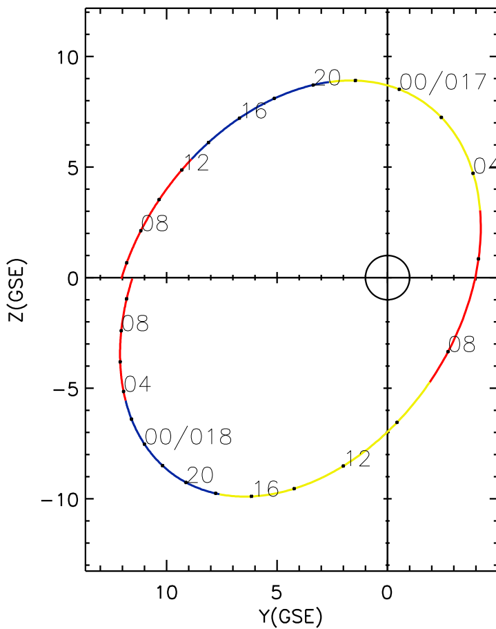
CLUSTER 2 orbit 2018 016 (01/16) 05:01 UT to 2018 018 (01/18) 11:16 UT
