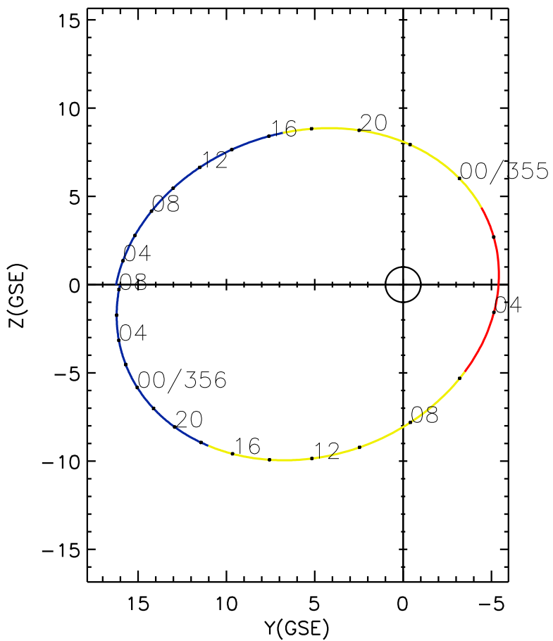
CLUSTER 2 orbit 2017 354 (12/20) 02:06 UT to 2017 356 (12/22) 08:21 UT
