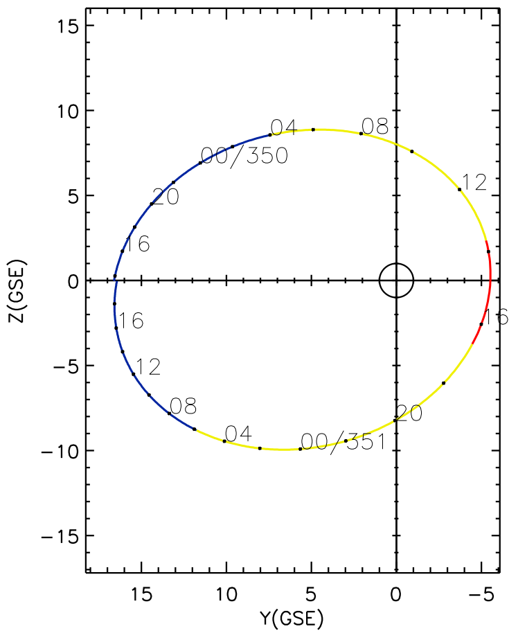
CLUSTER 2 orbit 2017 349 (12/15) 13:36 UT to 2017 351 (12/17) 19:51 UT
