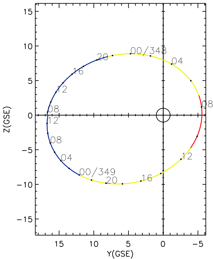
CLUSTER 2 orbit 2017 347 (12/13) 07:21 UT to 2017 349 (12/15) 13:36 UT
