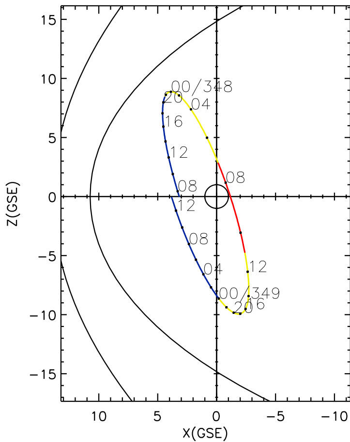
CLUSTER 2 orbit 2017 347 (12/13) 07:21 UT to 2017 349 (12/15) 13:36 UT
