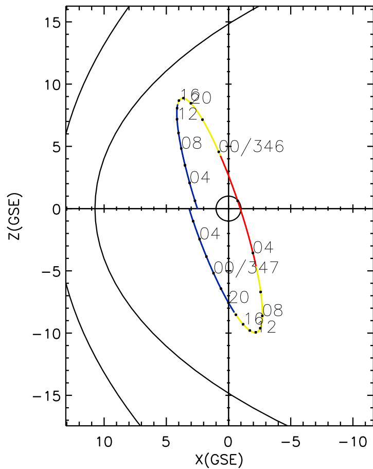
CLUSTER 2 orbit 2017 345 (12/11) 01:06 UT to 2017 347 (12/13) 07:21 UT
