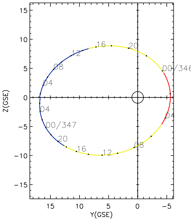
CLUSTER 2 orbit 2017 345 (12/11) 01:06 UT to 2017 347 (12/13) 07:21 UT
