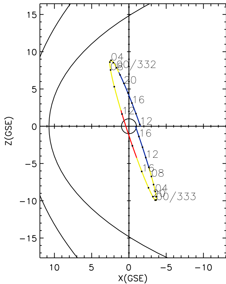
CLUSTER 2 orbit 2017 331 (11/27) 11:36 UT to 2017 333 (11/29) 17:51 UT
