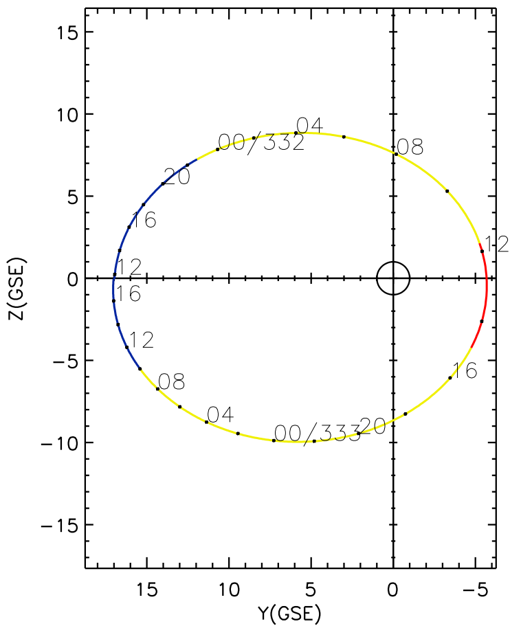
CLUSTER 2 orbit 2017 331 (11/27) 11:36 UT to 2017 333 (11/29) 17:51 UT
