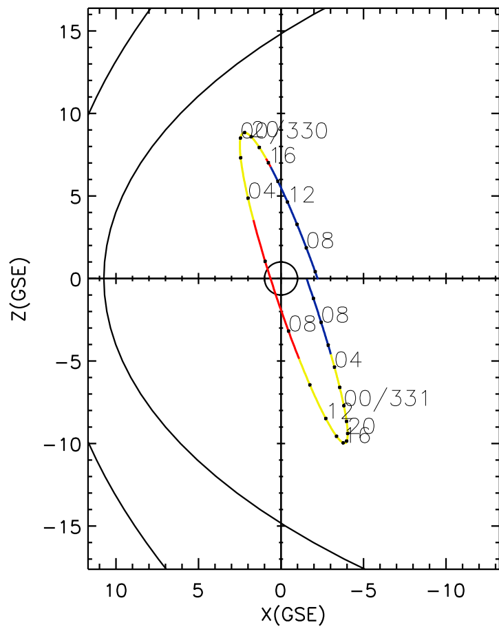
CLUSTER 2 orbit 2017 329 (11/25) 05:21 UT to 2017 331 (11/27) 11:36 UT
