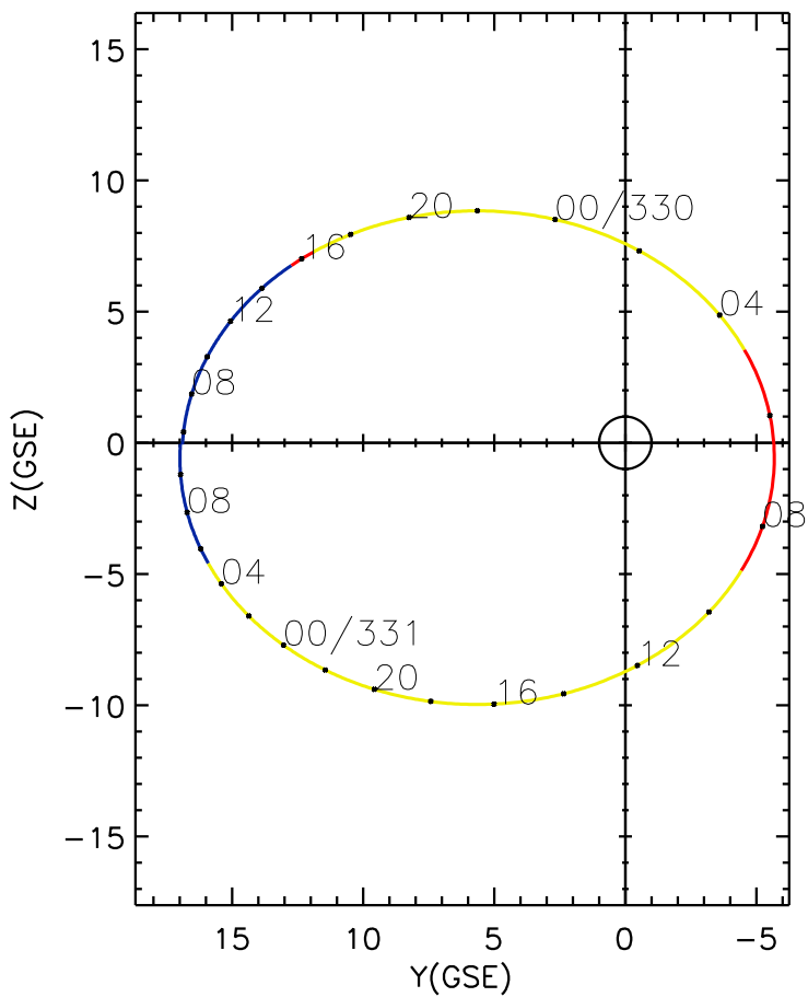
CLUSTER 2 orbit 2017 329 (11/25) 05:21 UT to 2017 331 (11/27) 11:36 UT
