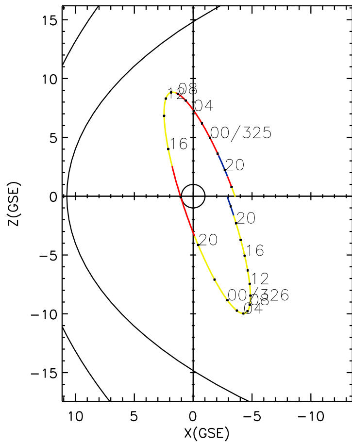
CLUSTER 2 orbit 2017 324 (11/20) 16:51 UT to 2017 326 (11/22) 23:06 UT
