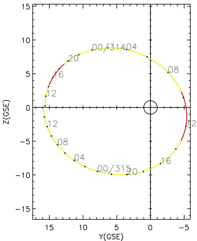
CLUSTER 2 orbit 2017 313 (11/09) 09:41 UT to 2017 315 (11/11) 15:56 UT
