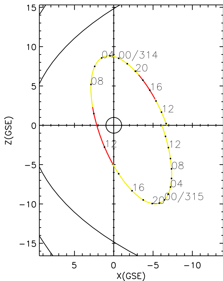
CLUSTER 2 orbit 2017 313 (11/09) 09:41 UT to 2017 315 (11/11) 15:56 UT
