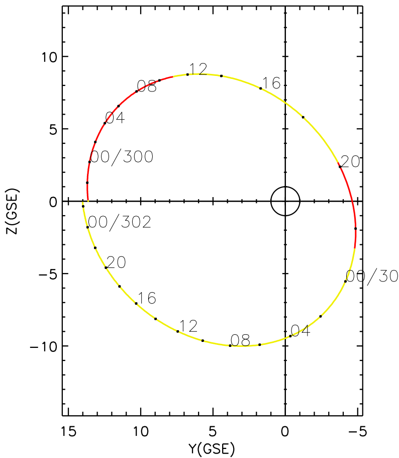
CLUSTER 2 orbit 2017 299 (10/26) 20:11 UT to 2017 302 (10/29) 02:26 UT
