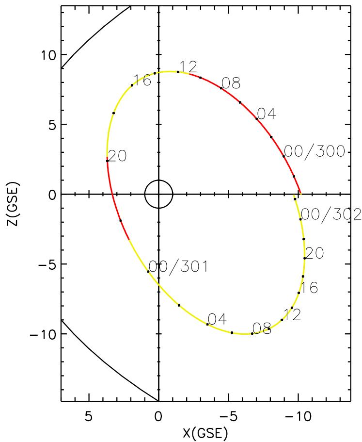
CLUSTER 2 orbit 2017 299 (10/26) 20:11 UT to 2017 302 (10/29) 02:26 UT
